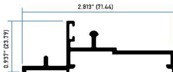
8371 Riel C/Mosquitero Interior
