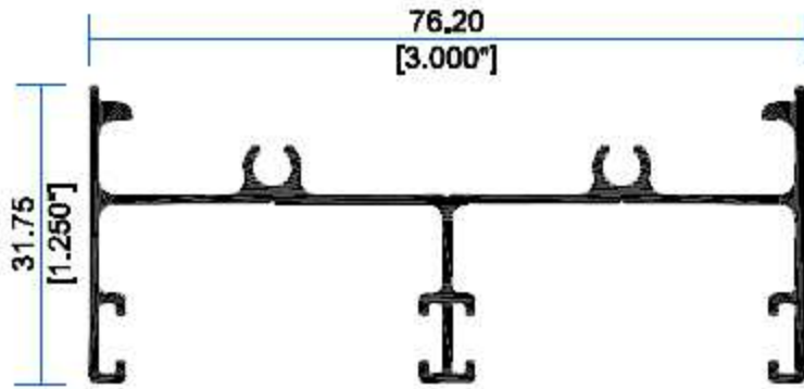
7826 Jamba
