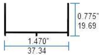
V17626 Jamba Lateral 6mm
