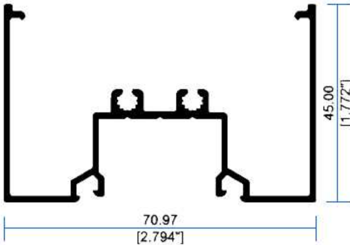
22592 Bolsa Duo
