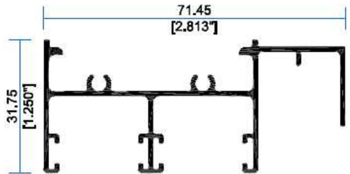
7819 Jamba C/Mosquitero
