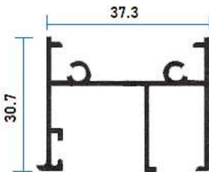
311037 Jamba
