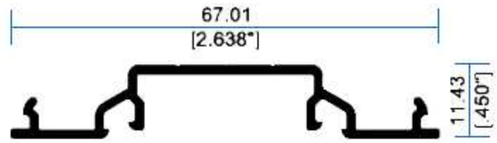
22594 Tapa Bolsa Duo
