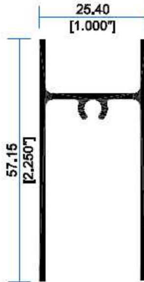
9960 Zoclo Ventana Duo
